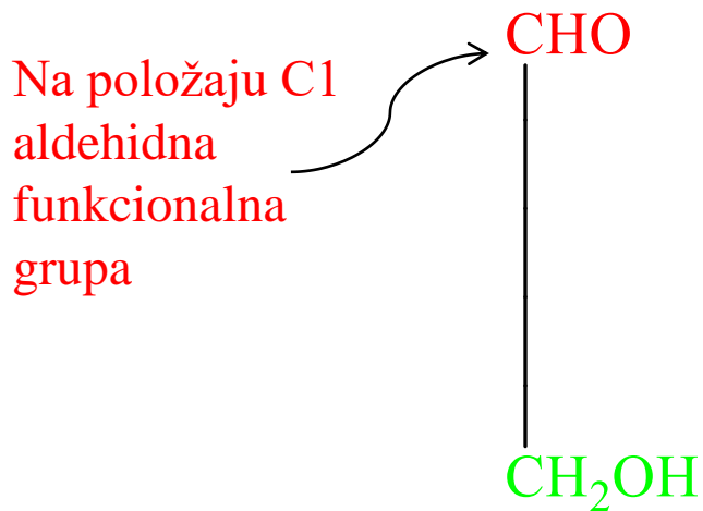
aldoze
