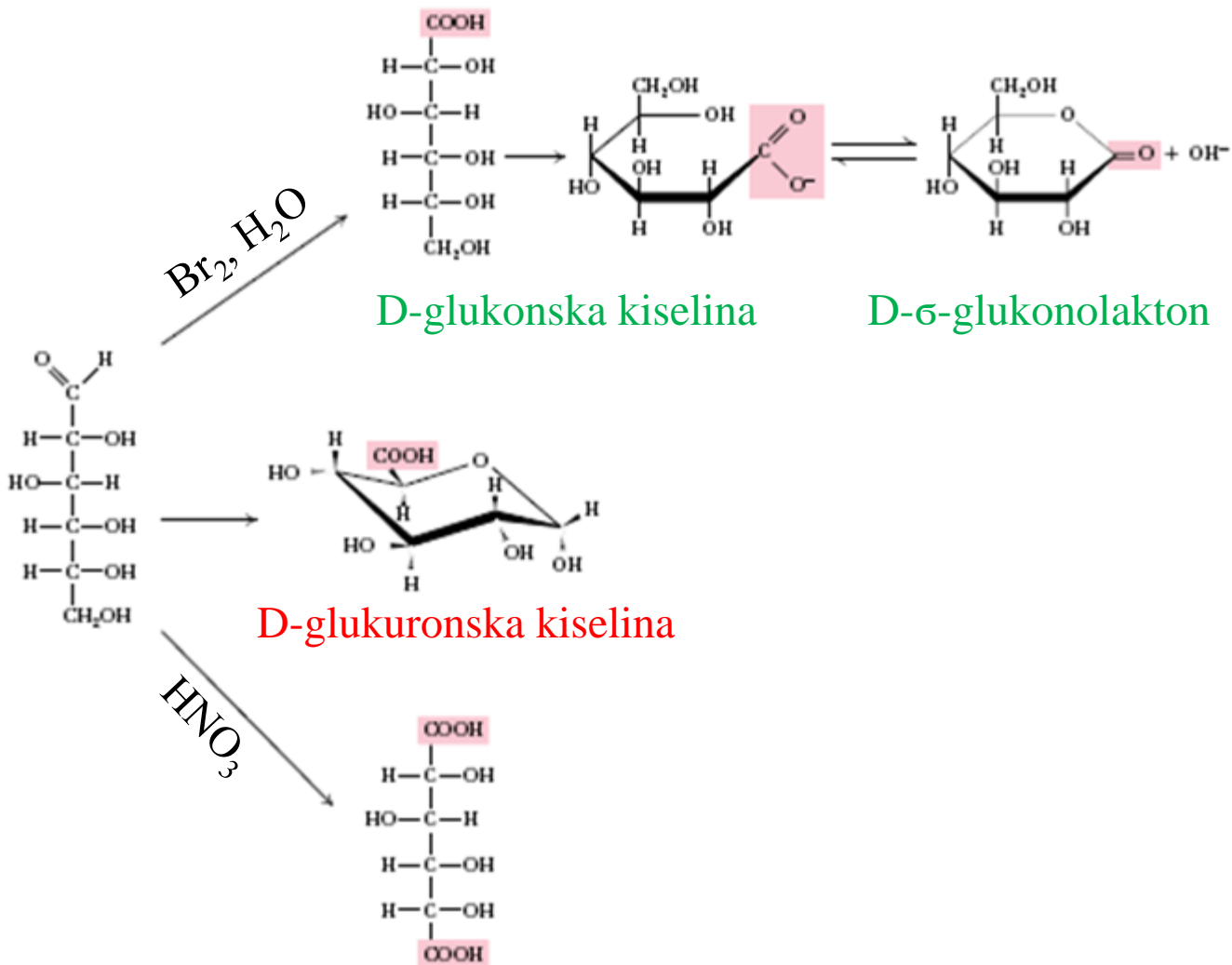
D-glukarna kiselina
